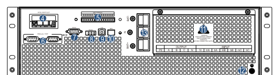
30kVA back appearance
